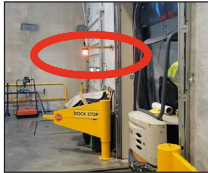
Dock Door Monitor activates and stays active while a forklift is in a truck
