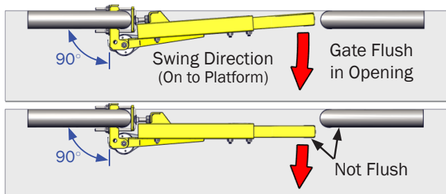
FINISHED GATE TOP VIEW
